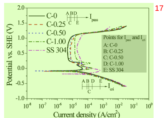
Fig. 1. Polarization diagrams for alloys C- x and SS 304 at 25^\circ\text{C} . 18
