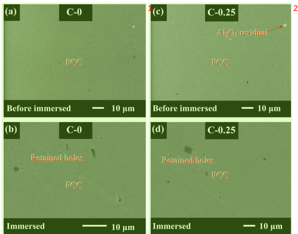
Fig. 11. Metallograph of alloys C-0 (a and b) and C-0.25 (c and d). (a) and (c), before; and (b) and (d), after immersion. Retained holes were from cast procedure, and Al 2 O 3 residuals were from polishing procedure.
