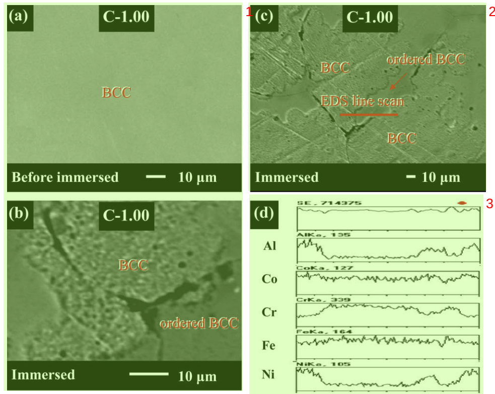
Fig. 13. Metallograph of alloy C-1.00. (a), before; (b) and (c), after immersion; and (d), EDS line-scan results of the location indicated in (c).
