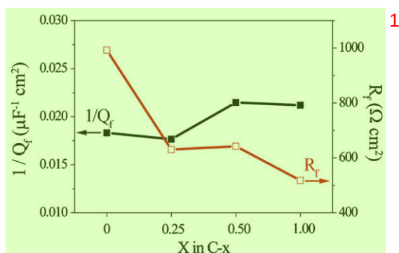
Fig. 7. Impedance and relative thickness ( 1/Q_f ) of oxide layer vs. Al content x plots.
