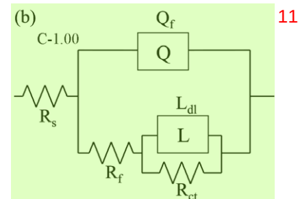
Fig. 6. EIS equivalent circuits (a) for alloys C-0, C-0.25, and C-0.50, and (b) for alloy C-1.00.
