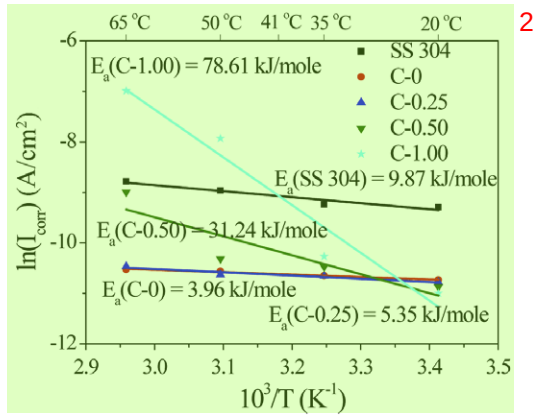
Fig. 4. The Arrhenius plots for alloys C-x and SS 304 at 20–65 °C.
