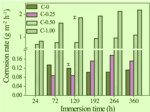
Fig. 2. Diagram showing change in corrosion rate (g m −2 h −1 ) in the 15-day-dipping and weight loss measurement for alloys C-x. 4
