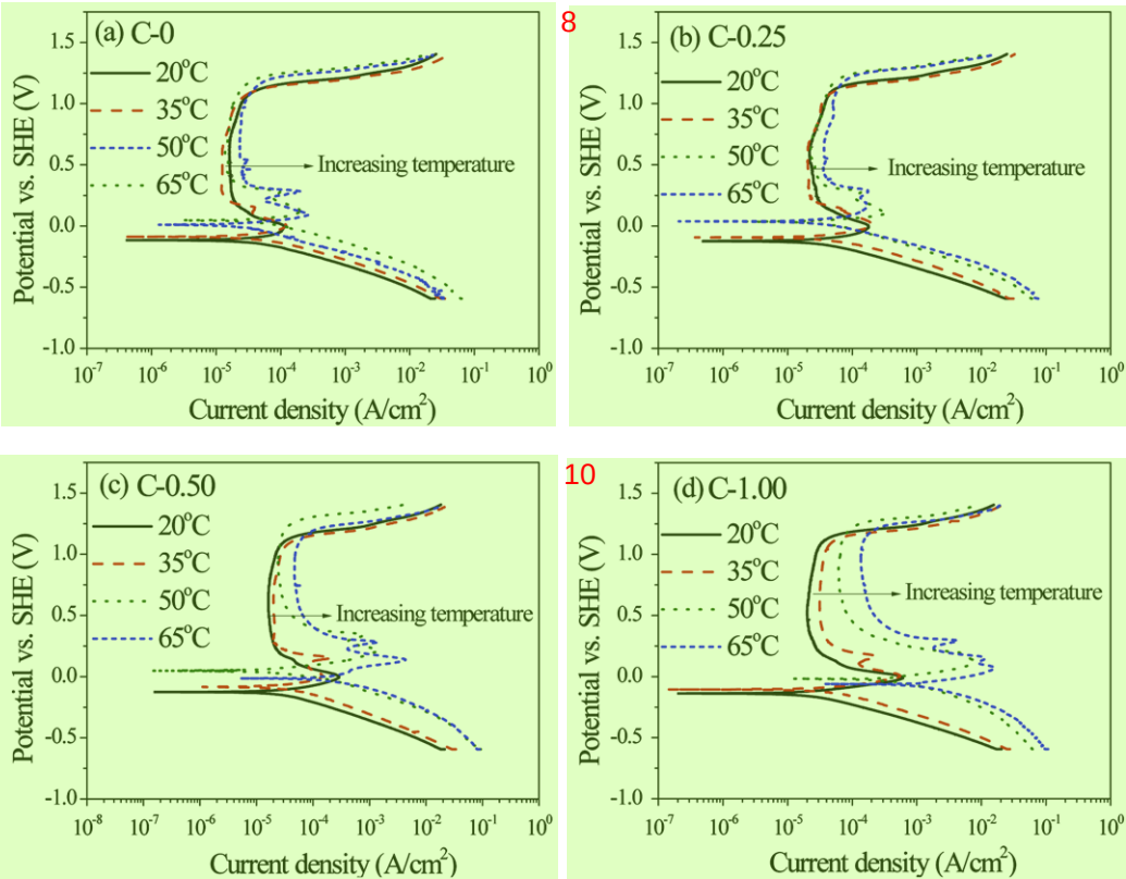
Fig. 3. Polarization diagrams for (a) C-0, (b) C-0.25, (c) C-0.50, and (d) C-1.00 at various temperatures. 18
