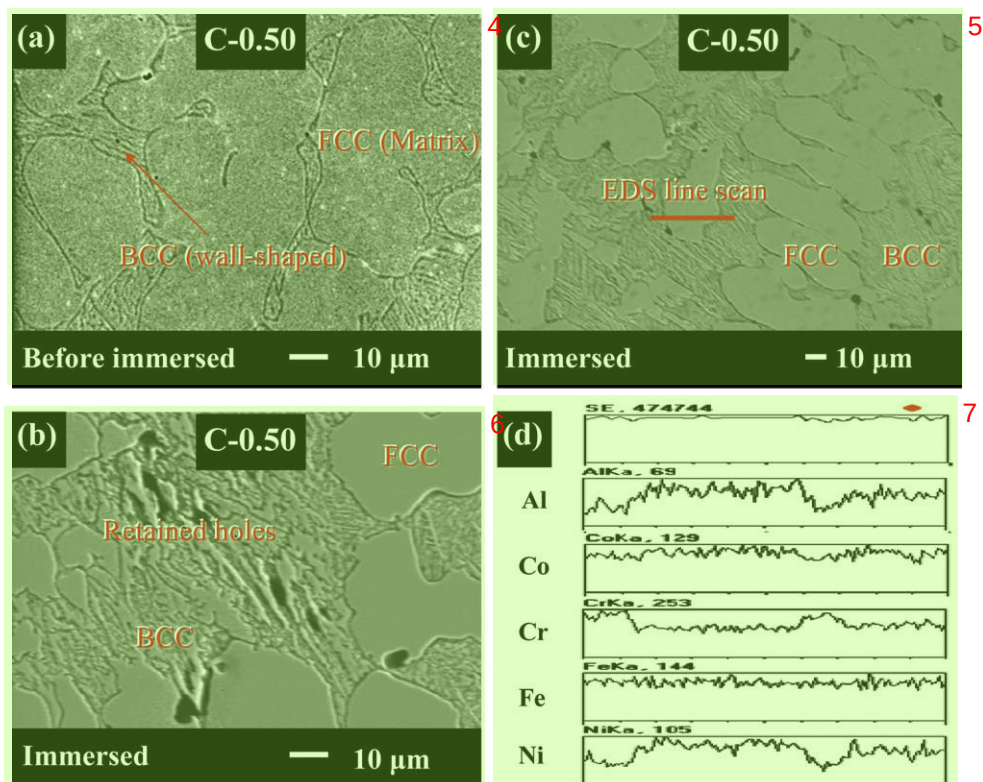
Fig. 12. Metallograph of alloy C-0.50. (a), before; (b) and (c), after immersion; and (d), EDS line-scan results of the location indicated in (c). Retained holes were from cast procedure.
