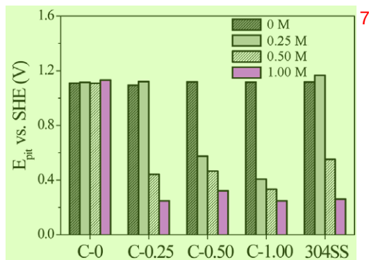
Fig. 10. Histogram of E_{\text{pit}} for alloys C-x and SS 304 in solution of different \text{Cl}^- ion molarity (M).
